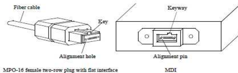
Figure 123-5—MPO-16 female two-row plug with flat interface, and an MDI
