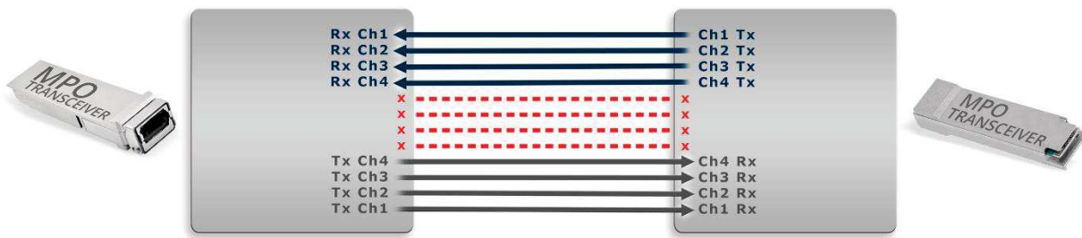
SR4 functional diagram
