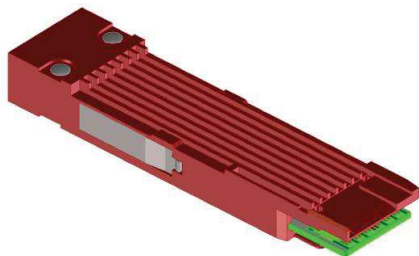
Figure 6c — QSFP-DD slotted top pluggable module rendering
